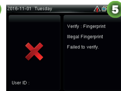
Verification fails
