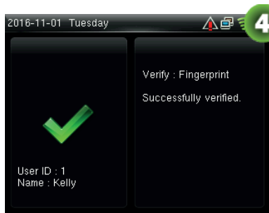
Verification succeeds
