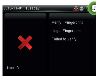
Verification fails
