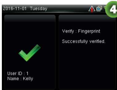
Verification succeeds
