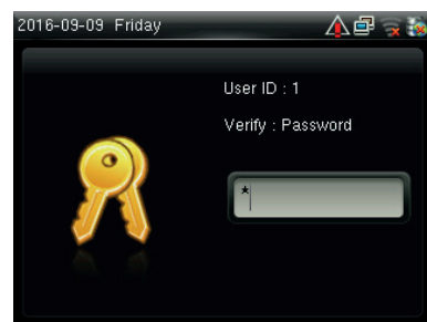
Input password
